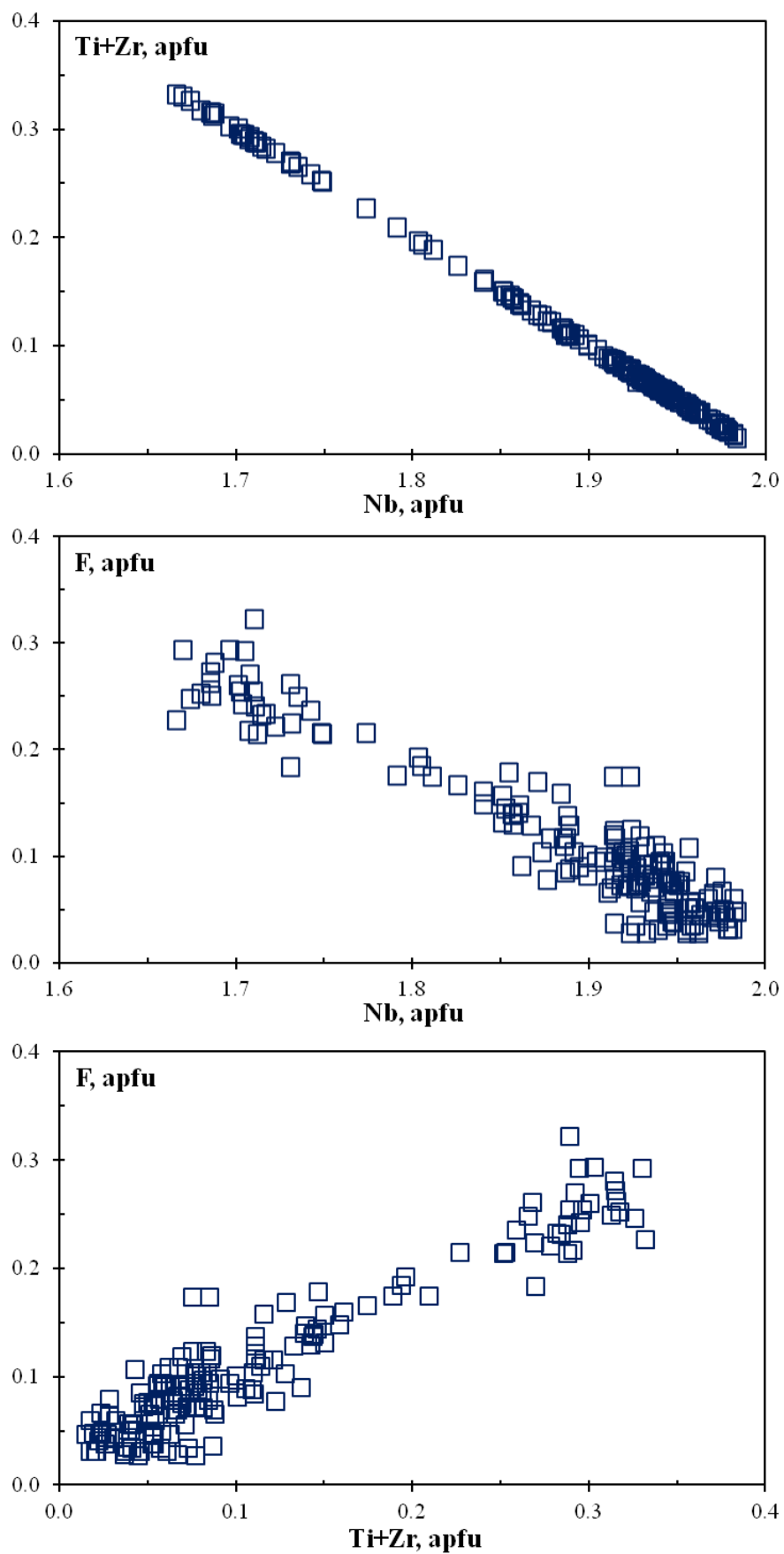
Figure 7. Compositional variations of rippite (in apfu).
