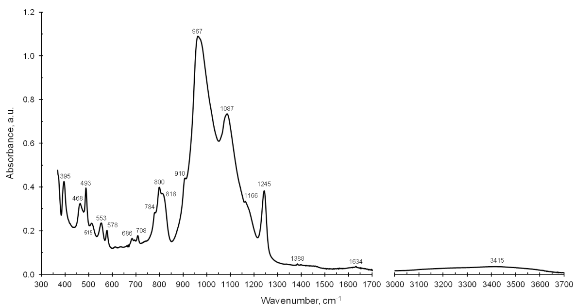
Figure 10. IR spectrum of rippite in the 350\text{--}1700 and 3000\text{--}3700\text{ cm}^{-1} ranges (powder KBr pellet).
