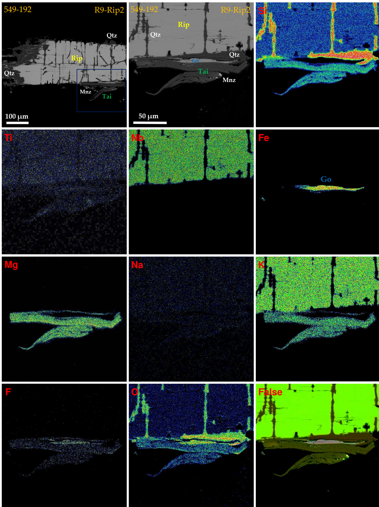
Figure S3. Relationship of rippite with tainiolite in the Chuktukon calciocarbonatite, BSE images and elemental maps. Symbols: Rip – rippite; Tai – tainiolite; Qtz – quartz, Go – goethite; Mnz – monazite-(Ce).
