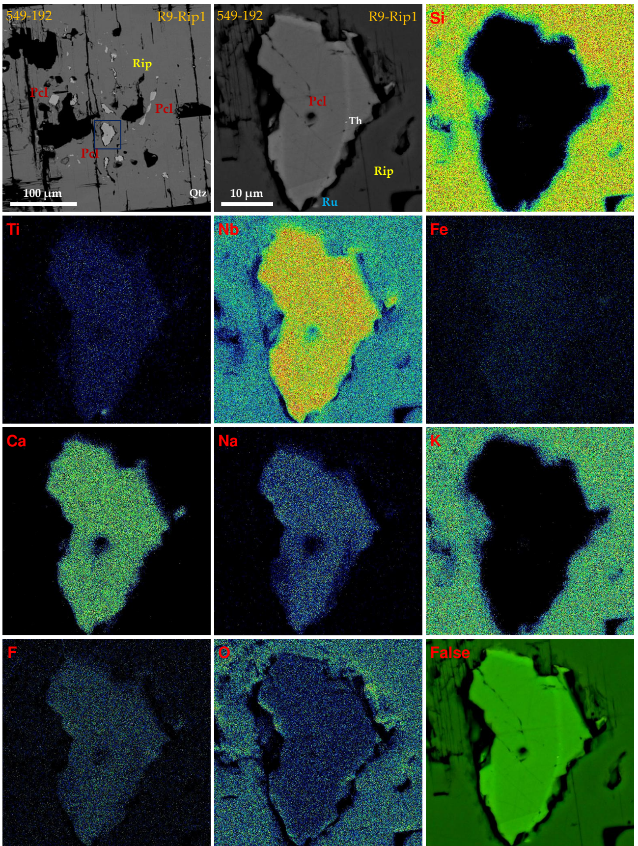
Figure S2. Inclusions of fluorcalciopyrochlore in rippite, Chuktukon calciocarbonatite, BSE images and elemental maps. Symbols: Rip – rippite; Pcl - fluorcalciopyrochlore; HPcl – Ba-Sr-Pb-rich hydro-/kenopyrochlore; Cpx – Ca-Na-rich clinopyroxene; Cc – calcite; Ru - rutile; Qtz – quartz, Th – thorite or thorianite. See also Figure 4.
