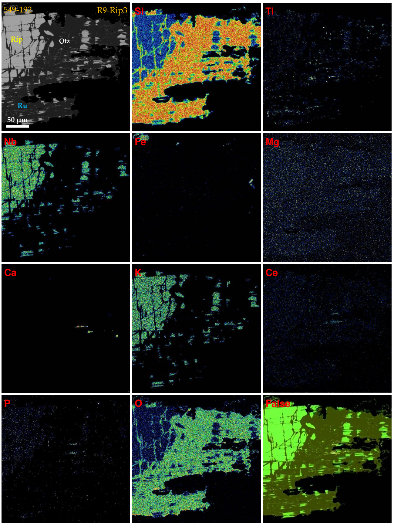
Figure S4. The outer zone in a rippite crystal and its replacement by quartz with formation of the \text{TiO}_2 phase (rutile ?), Chuktukon calciocarbonatite, BSE image and elemental maps. Symbols: Rip – rippite; Ru – rutile ?; Qtz – quartz.
