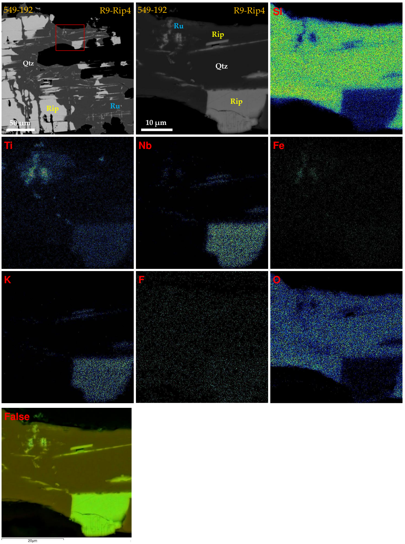
Figure S5. Replacement of rippite by quartz with formation of the \text{TiO}_2 phase (rutile ?), Chuktukon calciocarbonatite, BSE images and elemental maps. Symbols: Rip – rippite; Ru – rutile ?; Qtz – quartz.
