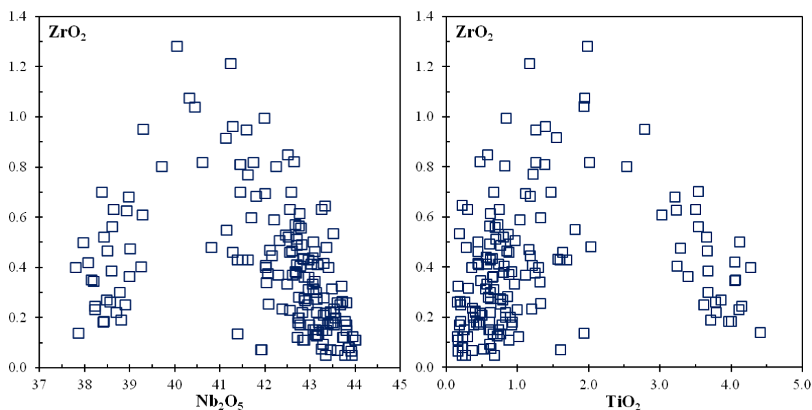
Figure 6. Variations of ZrO_2 versus Nb_2O_5 and TiO_2 in rippite (in wt %).
