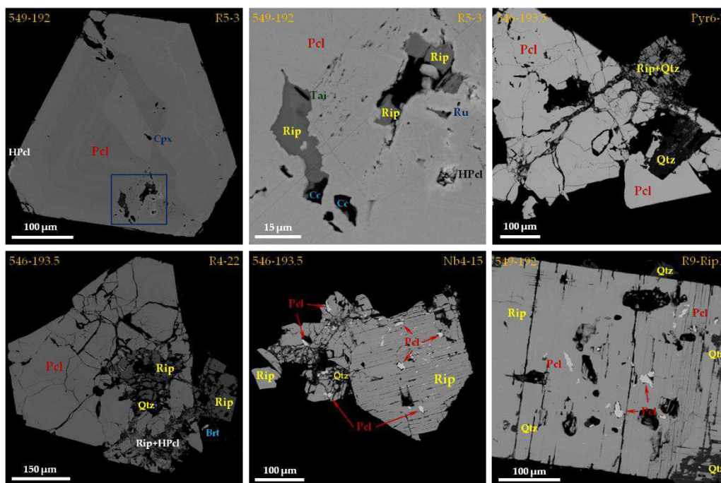
Figure 4. Relations between fluorcalciopyrochlore and rippite in the Chuktukon calcicarbonatites, BSE images. Symbols: Rip—rippite; Pcl—fluorcalciopyrochlore; HPcl—Ba-Sr-Pb-rich hydro-/kenopyrochlore; Cpx—Ca-Na-rich clinopyroxene; Cc—calcite; Ru—rutile; Tai—tainiolite; Qtz—quartz; Brt—barite. For some details see Figures S1 and S2.
