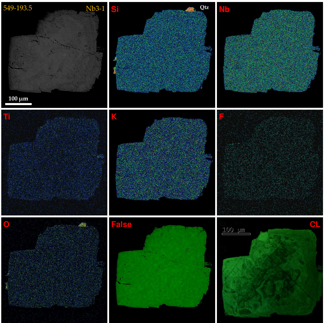
Figure S6. BSE and CL images and elemental maps for low-Ti rippite, Chuktukon calciocarbonatite. Symbols: Qtz – quartz.
