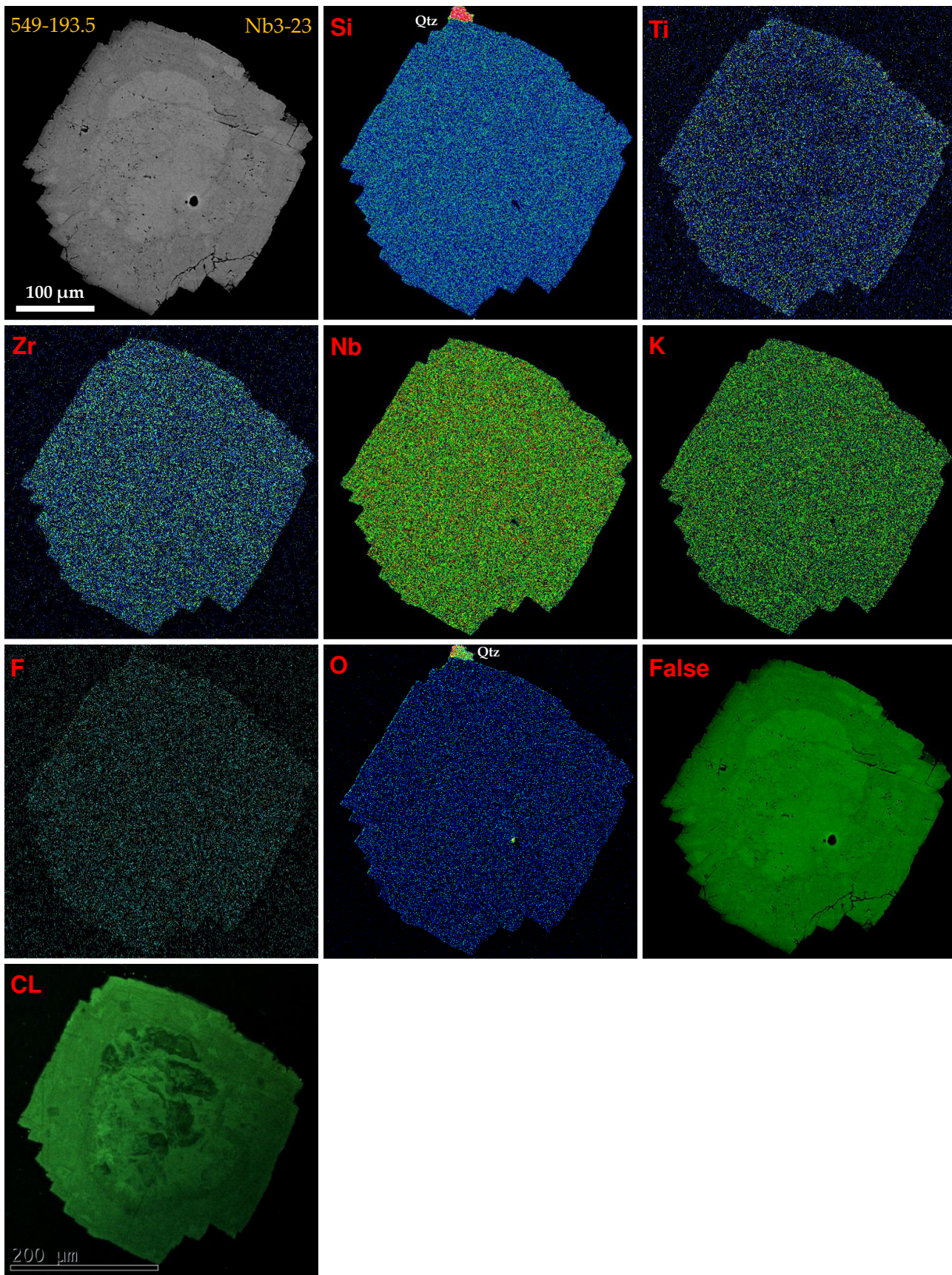
Figure S7. BSE and CL images and elemental maps for low-Ti rippite, Chuktukon calciocarbonatite. Symbols: Qtz – quartz.
