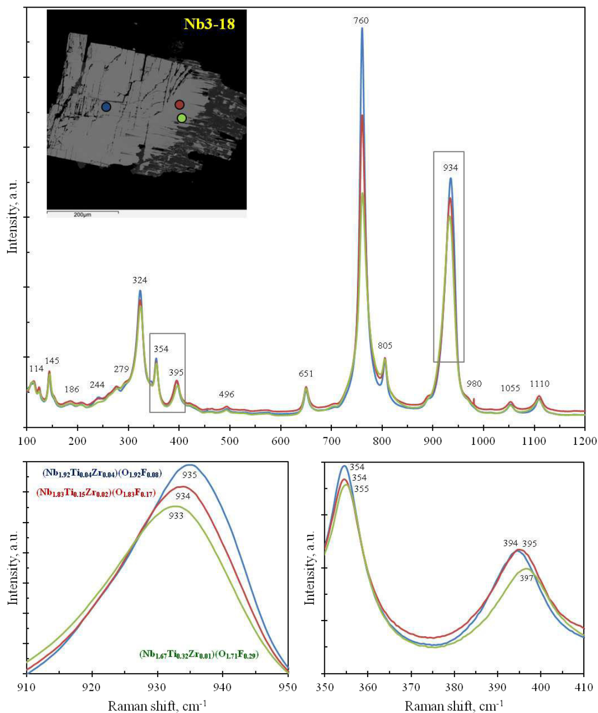
Figure 13. Raman spectra for a zoned rippite crystal showing dependence of some bands on chemical composition. For some details see Figures 5 and 8 and Tables 2 and S1.
