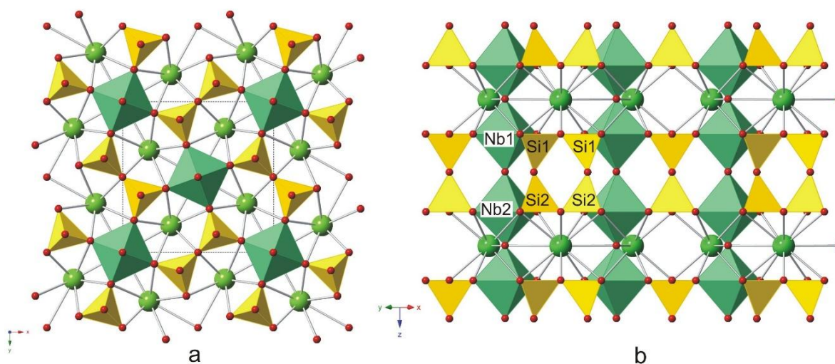
Figure 14. The crystal structure of rippite in (001) (a) and (110) (b) projections. Large green balls—K; small red balls—O.
