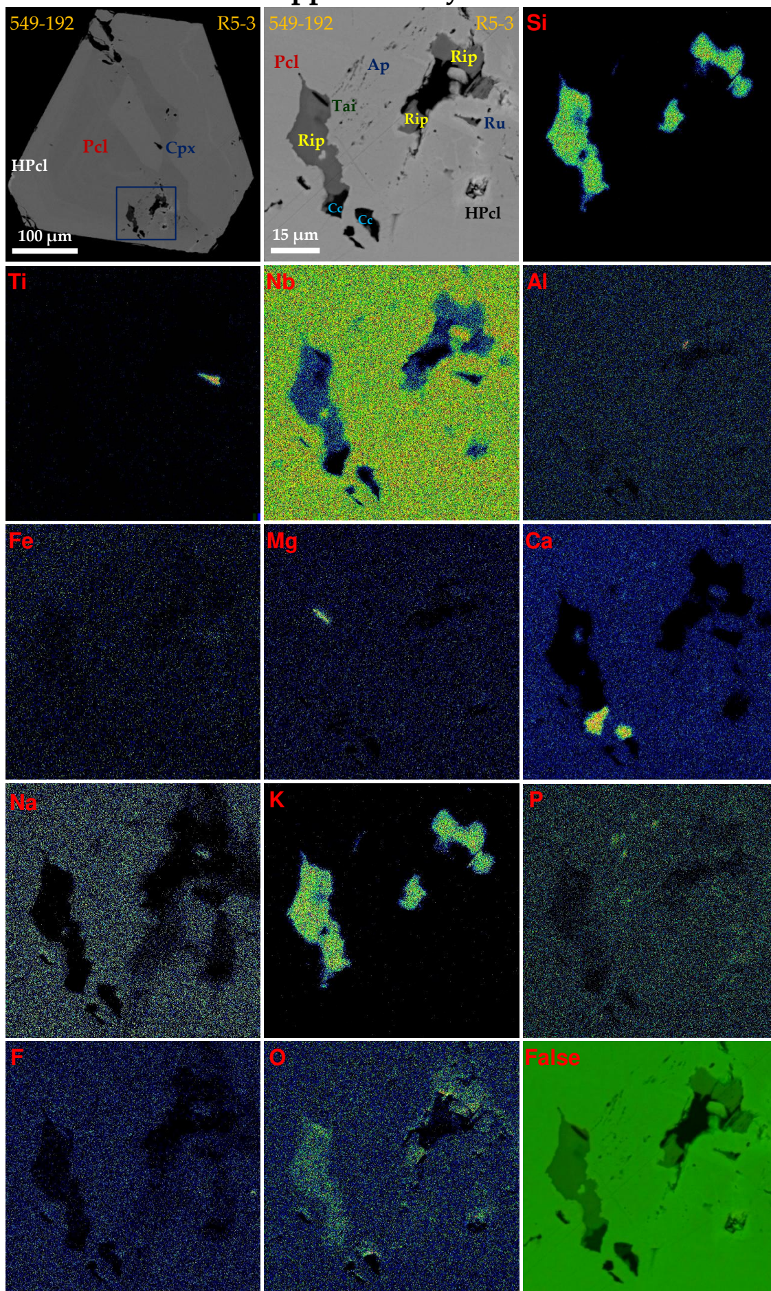
Figure S1. Secondary polymineral inclusions with rippite in fluorcalciopyrochlore, Chuktukon calciocarbonatite, BSE images and elemental maps. Symbols: Rip – rippite; Pcl - fluorcalciopyrochlore; HPcl – Ba-Sr-Pb-rich hydro-/kenopyrochlore; Cpx – Ca-Na-rich clinopyroxene; Cc – calcite; Ru - rutile; Tai – tainiolite; Qtz – quartz. See also Figure 4.
