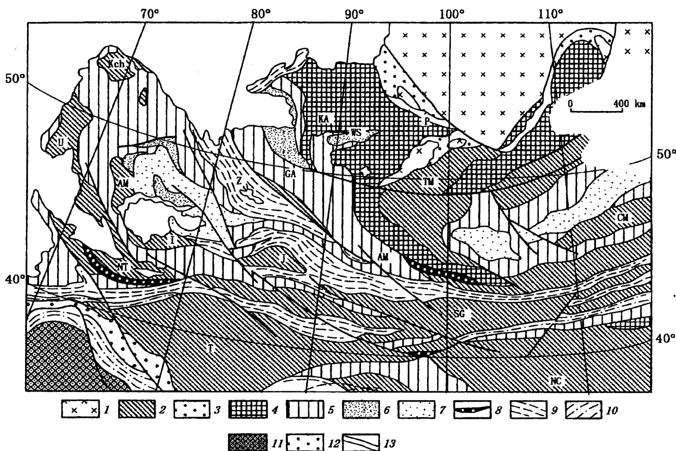
Fig. 2. The tectonic scheme of the Central Asian foldbelt (Mossakovsky et al., 1993). 1, 2=platforms and microcontinents: 1=Siberian platform, 2=Gondwana group (T=Tarim and NC=North China platforms, Kch=Kokchetav, U=Ulutau, AM=Aktai-Mointin, I=Ili, NT=North Tian Shan, J=Junggar, TM=Tuva-Mongolian, CM=Central Mongolian, and SG=South Gobi microcontinents); 3–5=accretionary zones: 3=Late Riphean, 4=Salair? Funny? (KA=Kuznetsk Alatau, WS=West Sayan), 5=Caledonian (S=Salair, GA=Gorny Altai, AM=Altai-Mongolian); 6, 7=sedimentary basins: 6=Caledonian (Anui-Chuya), 7=Early Hercynian; 8–11=collisional foldbelts: 8=Caledonian, 9=Early Hercynian (Z=Zaisan), 10=Late Hercynian, 11=Mesozoic; 12=Predkunlun trough; 13=large faults.
