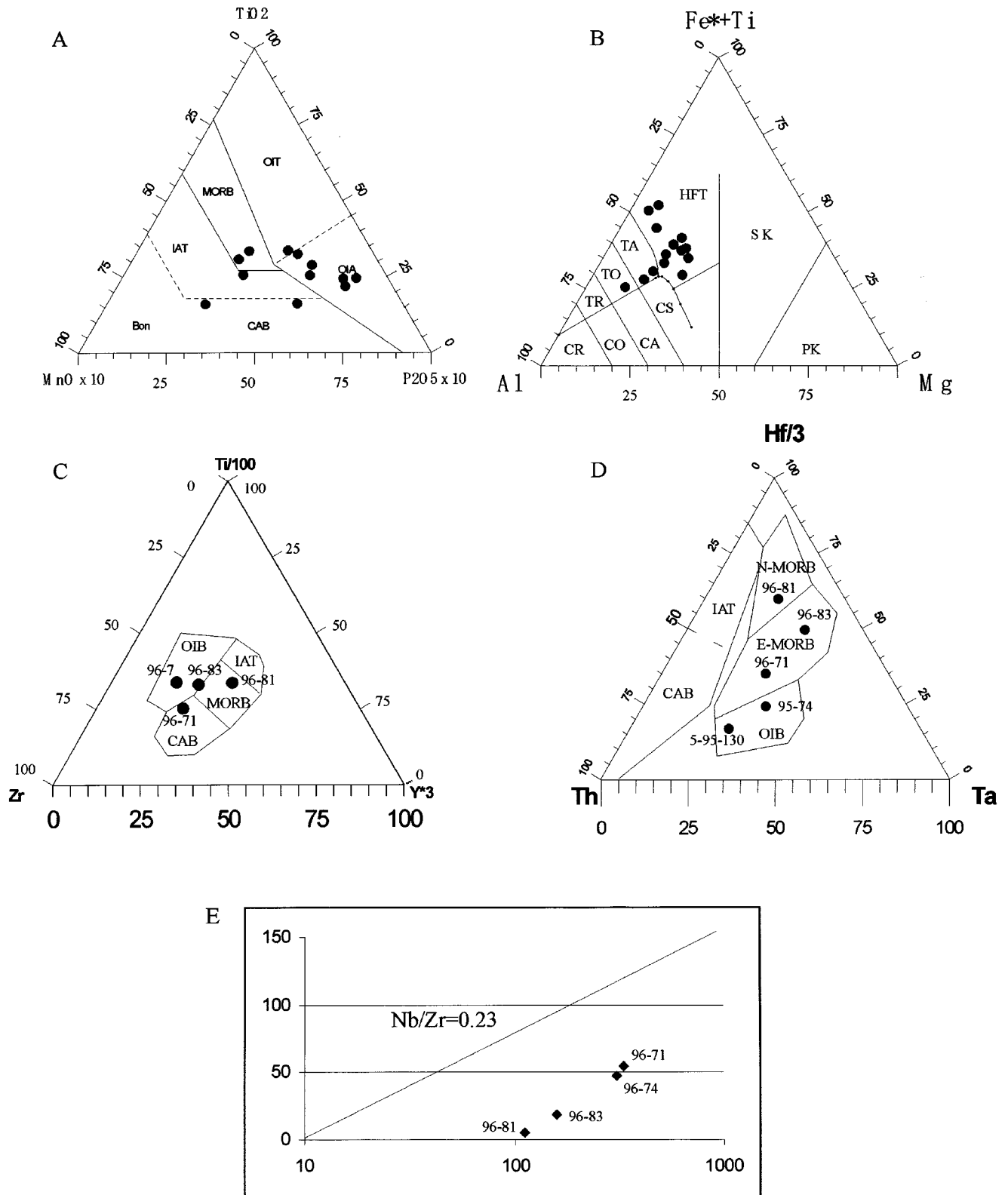
Fig. 6. Major and trace element concentrations in the Zasurin basaltoids: Al_2O_3-FeO+TiO_2-MgO classification diagram; discrimination diagrams: MnO-TiO_2-P_2O_5 , Th-Hf-Ta , Zr-Ti-Y ; Nb/Zr plot (definition of the fields see in Fig. 9).
