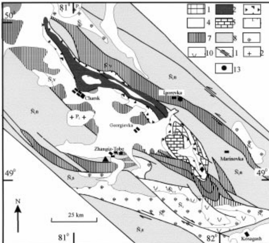
Fig. 8. The geological scheme of the Chara zone (modified from Abdulin and Patalakha, 1981). 1–6=oceanic crust units, 1=Early Paleozoic Type I serpentinitic mélangé with blocks of high-pressure rocks, 2=Ordovician Type II mélangé with blocks of weakly altered peridotites and gabbro, 3=Type III mélangé with blocks of Type I and II mélangé, Ordovician–Carboniferous oceanic crust and island arcs of the Kazakhstan and Siberian continents; 4–6=large fragments of oceanic crust: 4=Middle Devonian oceanic islands (basalt and chert), 5=Early–Middle Devonian seamounts (reef limestones), 6=Ordovician gabbro, 7=Visean–Namurian accretionary units with Middle Devonian–Early Carboniferous N-MORB and OIB, 8=Early Carboniferous fore-arc turbidites, Late Devonian–Early Carboniferous reef limestones, siliceous rocks and oceanic volcanogenic-siliceous rocks, 9–10=collisional units, 9=Late Carboniferous continental molasse, 10=Late Carboniferous alkaline volcanics, 11=Late Carboniferous–Early Permian strike-slip faults, 12=Late Permian–Early Triassic post-collisional granites.
